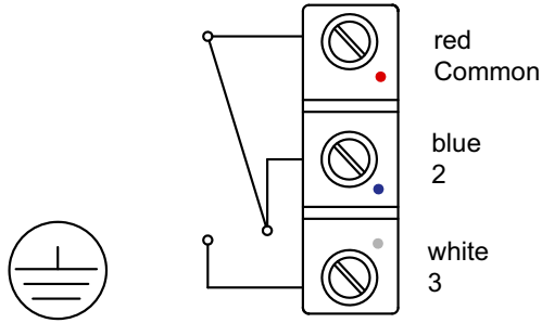
Fig. 3.2: Circuit diagram
