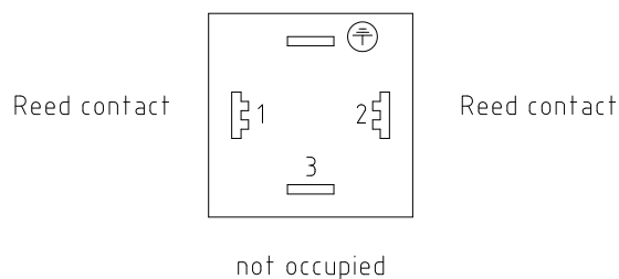
Fig 2: Circuit diagram
